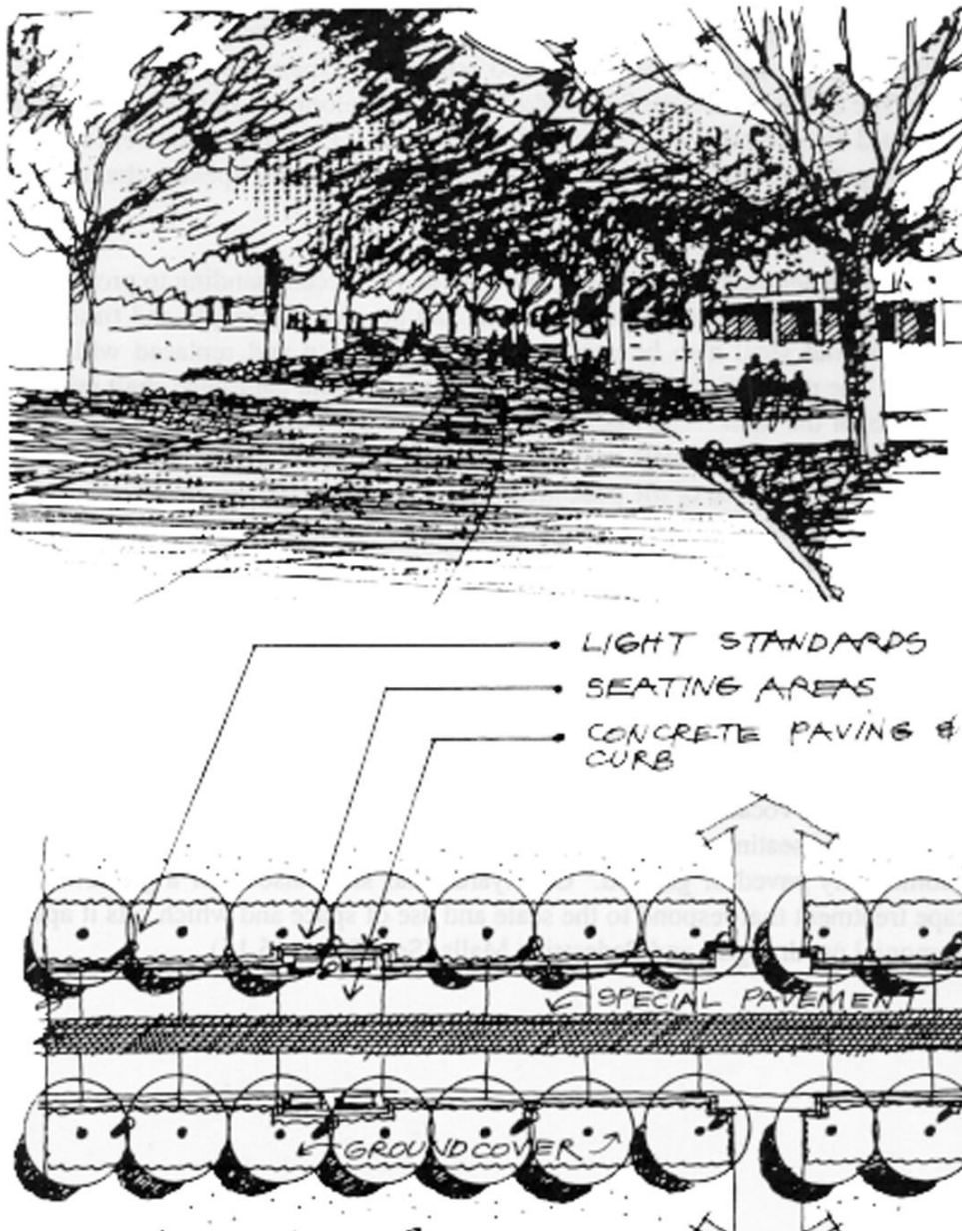
Figure 16.9 Pedestrian Corridor
